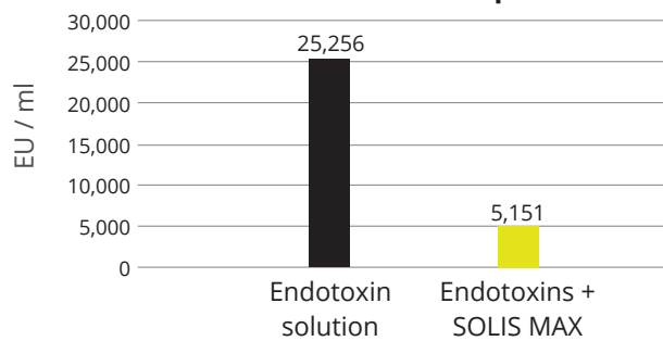
Endotoxin adsorption
